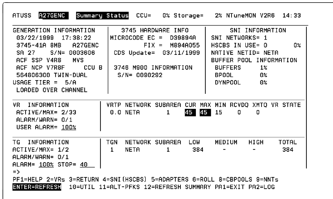
Figure 4-79. ATUSS Summary Status Panel
