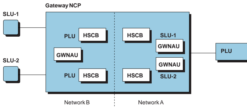
Figure 4-55. GWNAUs and HSCBs in a Gateway NCP
