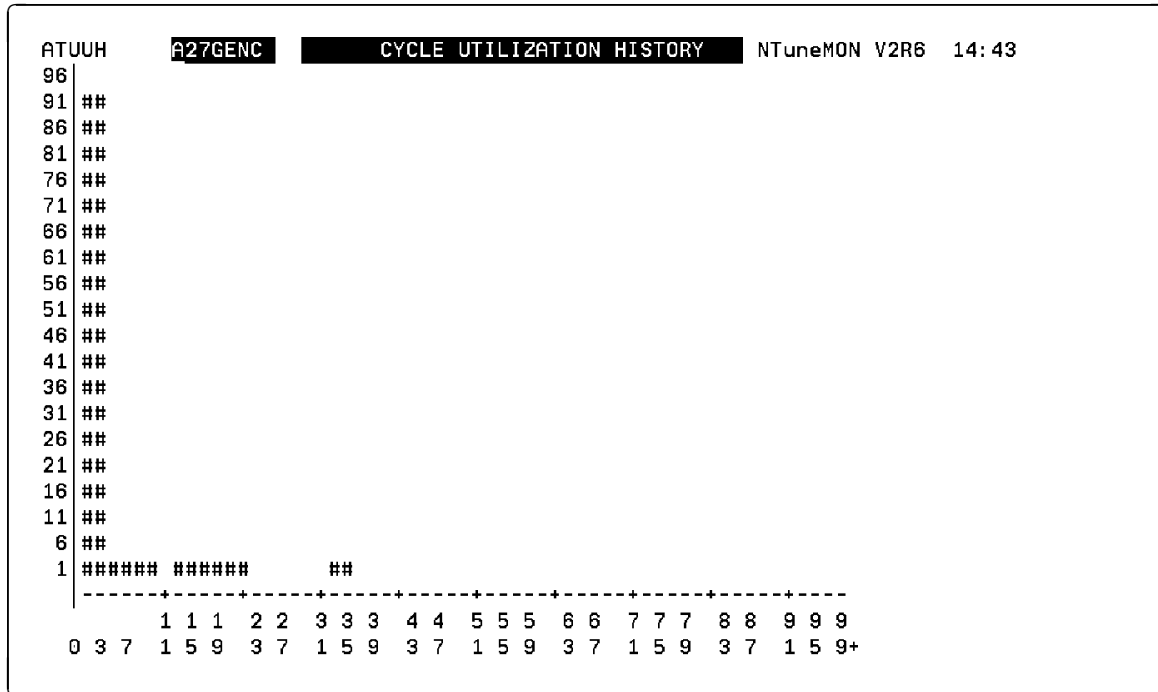
Figure 4-95. ATUUH Cycle Utilization History Panel
