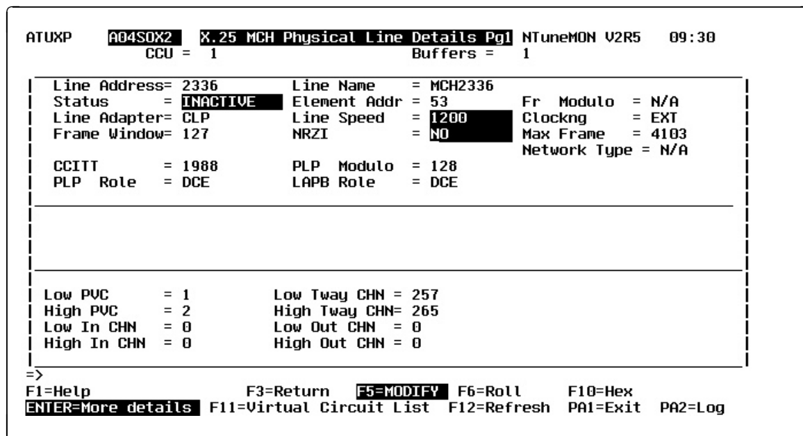
Figure 6-35. ATUXP X.25 MCH Physical Line Details Page 1 Panel for X.25 ODLC
