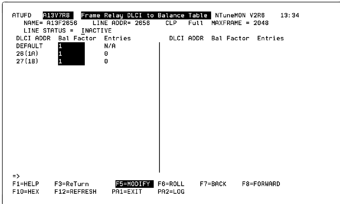
Figure 6-8. ATUFD Frame Relay DLCI to Balance Table Panel
